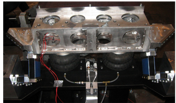
Mounting Table with Air Spring Load Support and Flexures for Fore-aft Excitation
