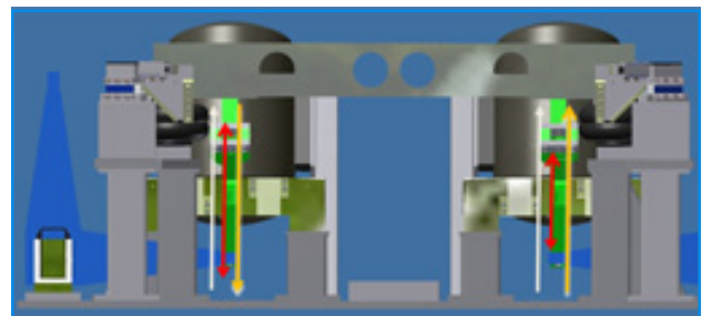
MISO: One Control, Both Shakers, Vertical, in-phase ↑↑ Roll, out-of-phase ↑↑ MIMO: Independent Control of each Shaker to Left-Side, Right-Side Drive Files ↑↑ Vertical & Roll controlled in one test ↑↑
