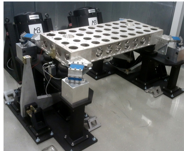
Vertical & Roll Excitation, 4 DOF Mode
